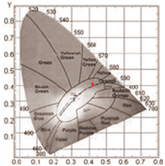
Chromaticity Diagram:
